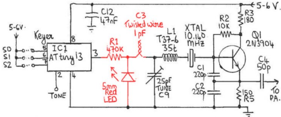
Original circuit diagram
