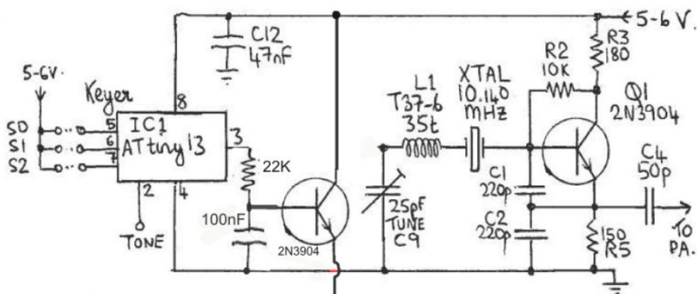
Mod circuit diagram
