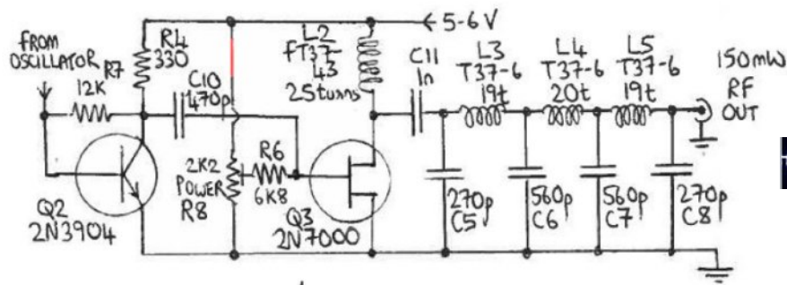
Mod circuit diagram
